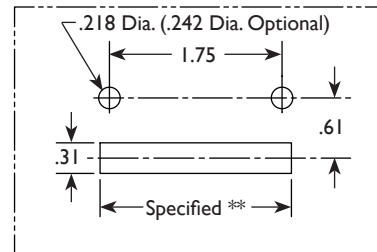
Panel Cutout Detail Sheetmetal Style Lever
