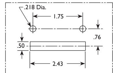
Panel Cutout Detail Rod Style Lever
